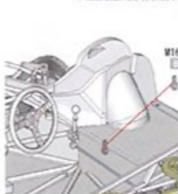
図の様に取付けます。 Please assemble as shown.
